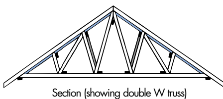
Diagram 2. Standard bracing for rafter and web members of duo-pitch trussed rafters.
