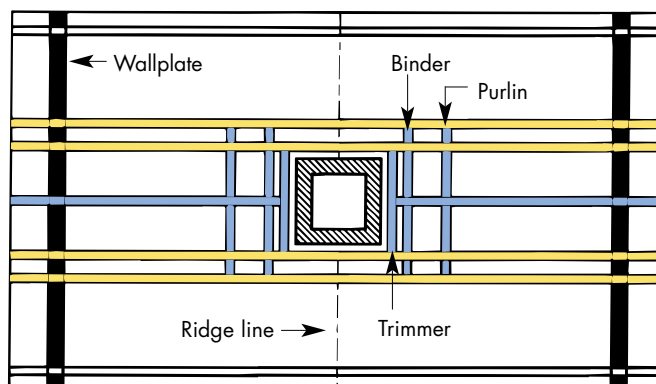
CHIMNEY DETAIL
