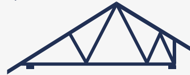
BOBTAIL / STUB END
